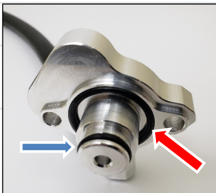
Figure 10: Install O-Rings
