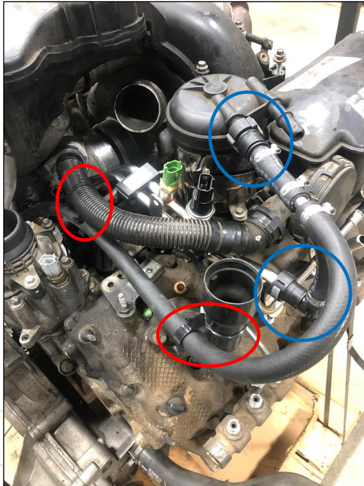
Figure 12: Hose Routing & Zip Tie locations
