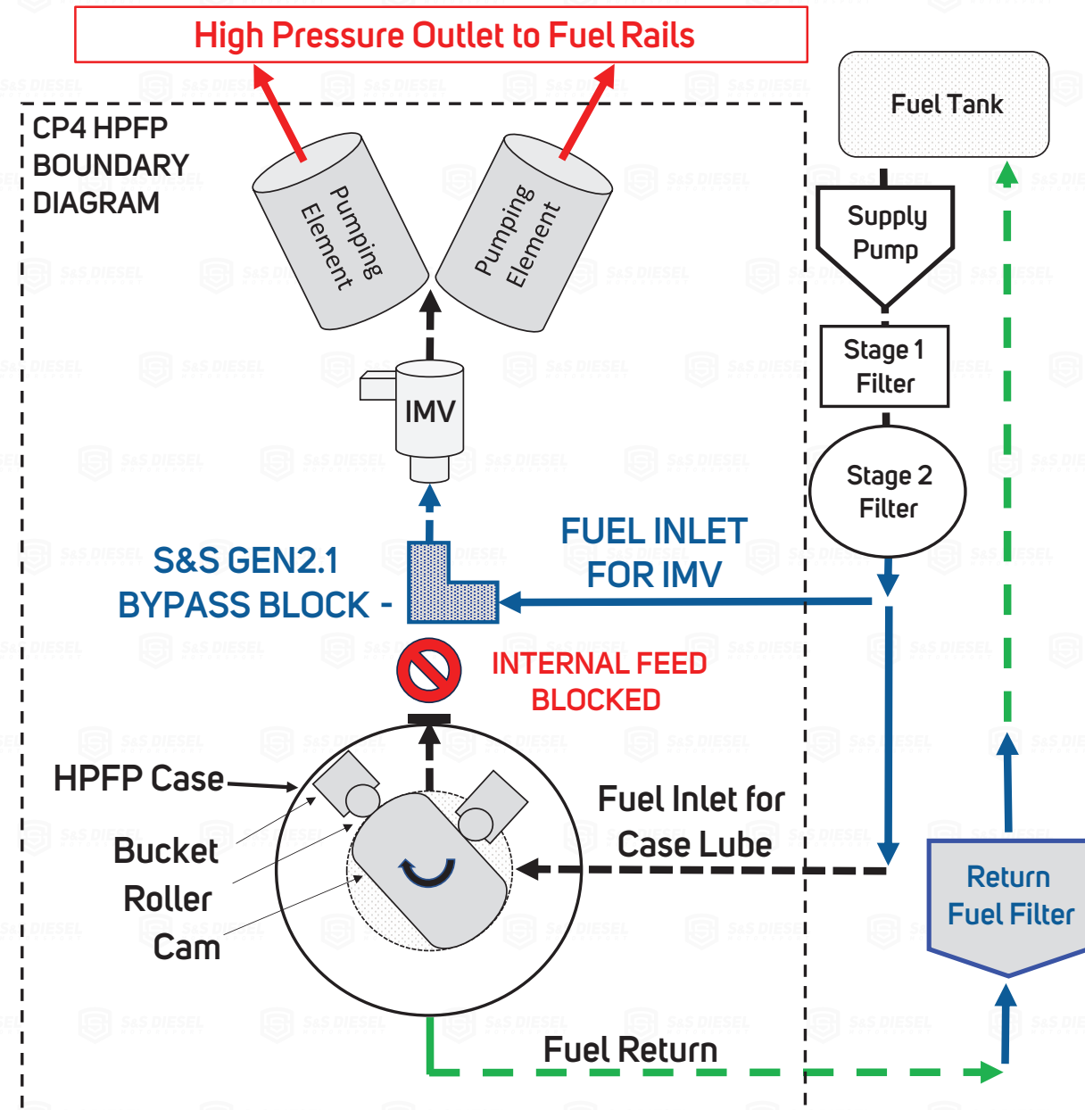
S&S GEN2.1 DPK FUEL FLOW DIAGRAM
