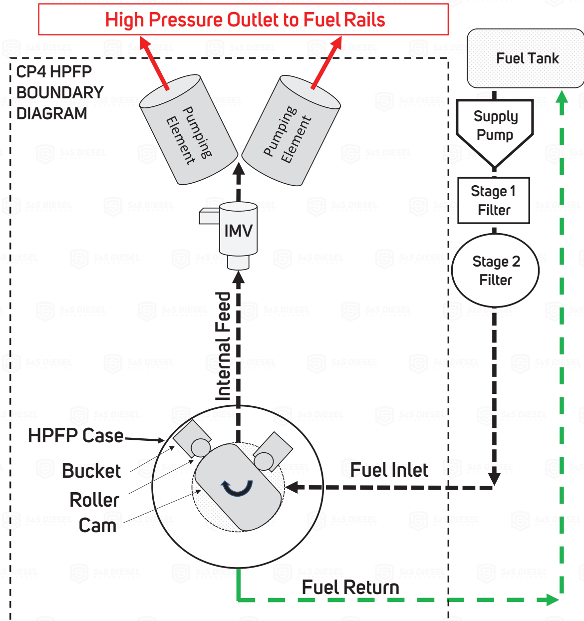
OEM FUEL FLOW DIAGRAM
